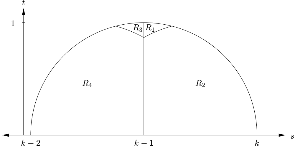
FIGURE 1. Decomposition of the region R in Proposition 7.5 into subregions.
